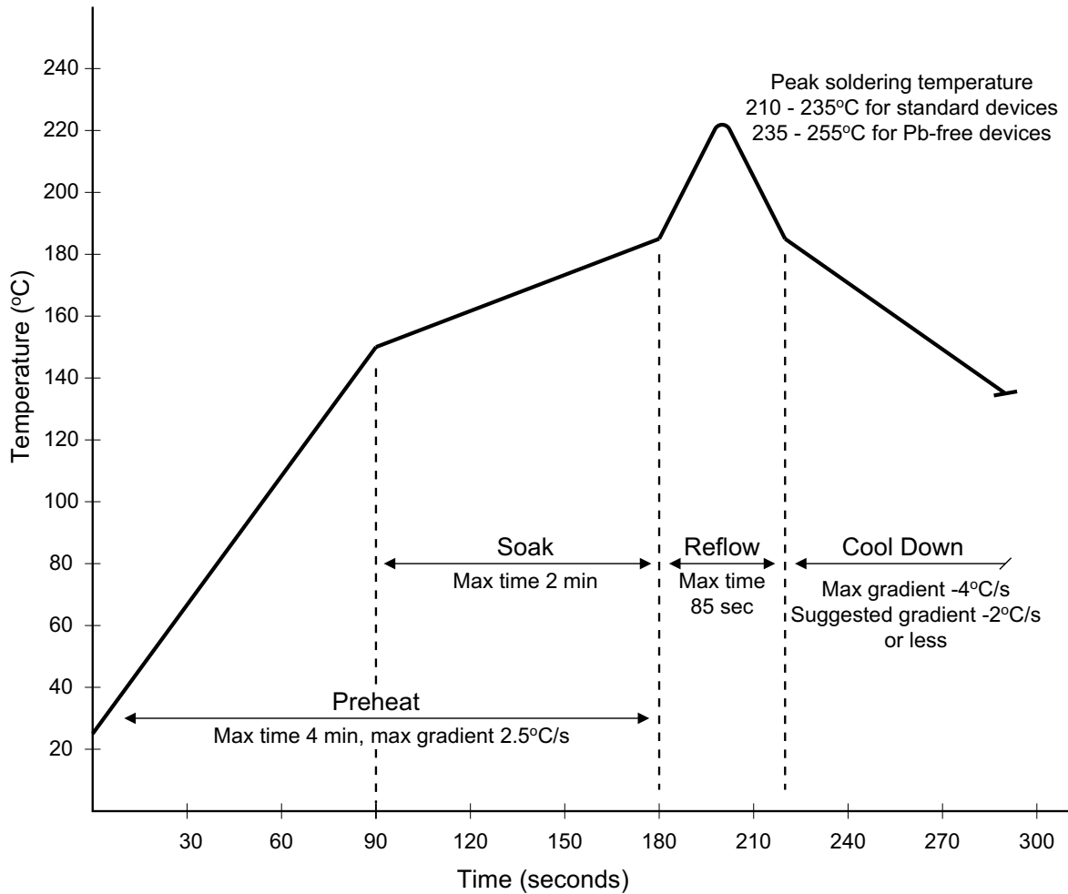
Fig. 10. Typical IR Reflow Soldering Thermal Profile
