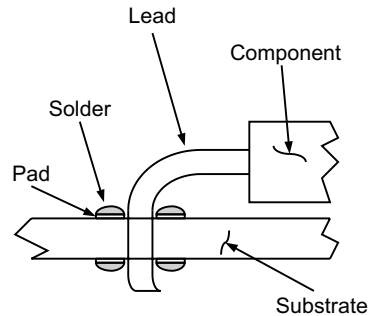
Fig. 8. Non-wetting Solder Joint
