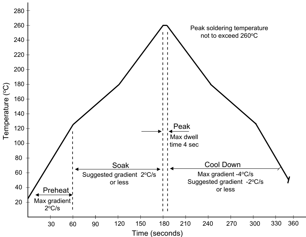
Fig. 9. Typical Wave Soldering Thermal Profile
