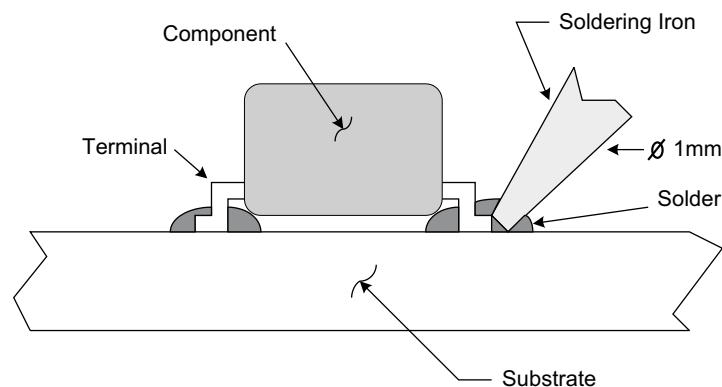
Fig. 11. Rework by Soldering Iron
